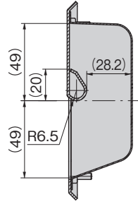
Reference cross section [A-1030-0]
