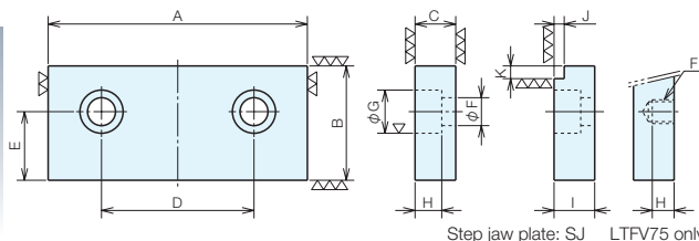
Step jaw plate: SJ LTFV75 only
