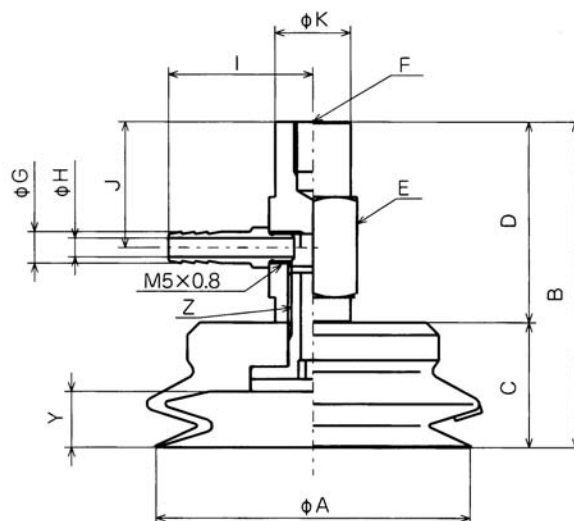
PJYK-10/15/20/25/30/35/40/50
