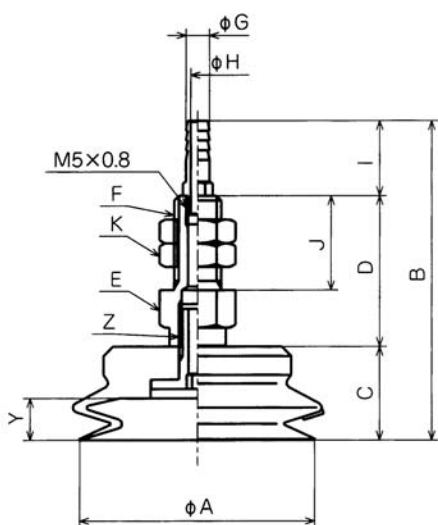
PJTK-10/15/20/25/30/35/40/50
