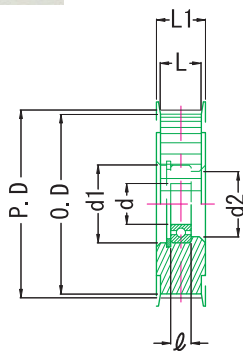
(TPI-037~TPI-100H)
