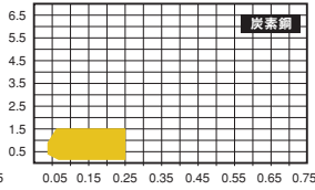
WNMG 06T304-SF
